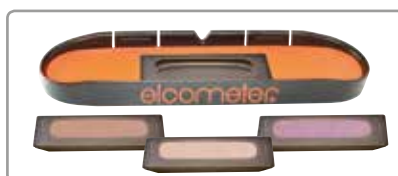
The soft material specimen holder is supplied with 3 sample trays - ideal for testing soft, powder or viscous materials
